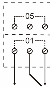
Internal connections of a single digital output
