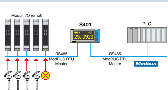
Controllo locale via PLC e I/O remoto
