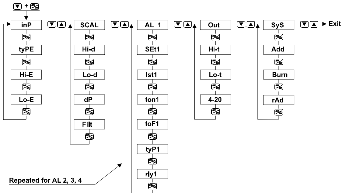
Diagram of the programming menu structure.
